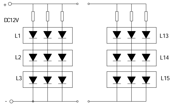
Circuit Diagram
