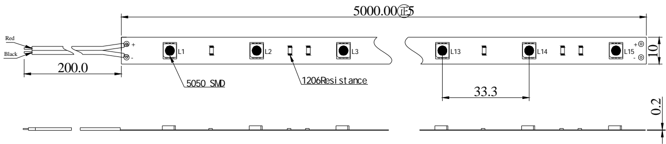
Dimension Drawing
