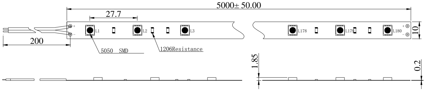
Dimension Drawing
